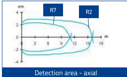
Detection area - axial
